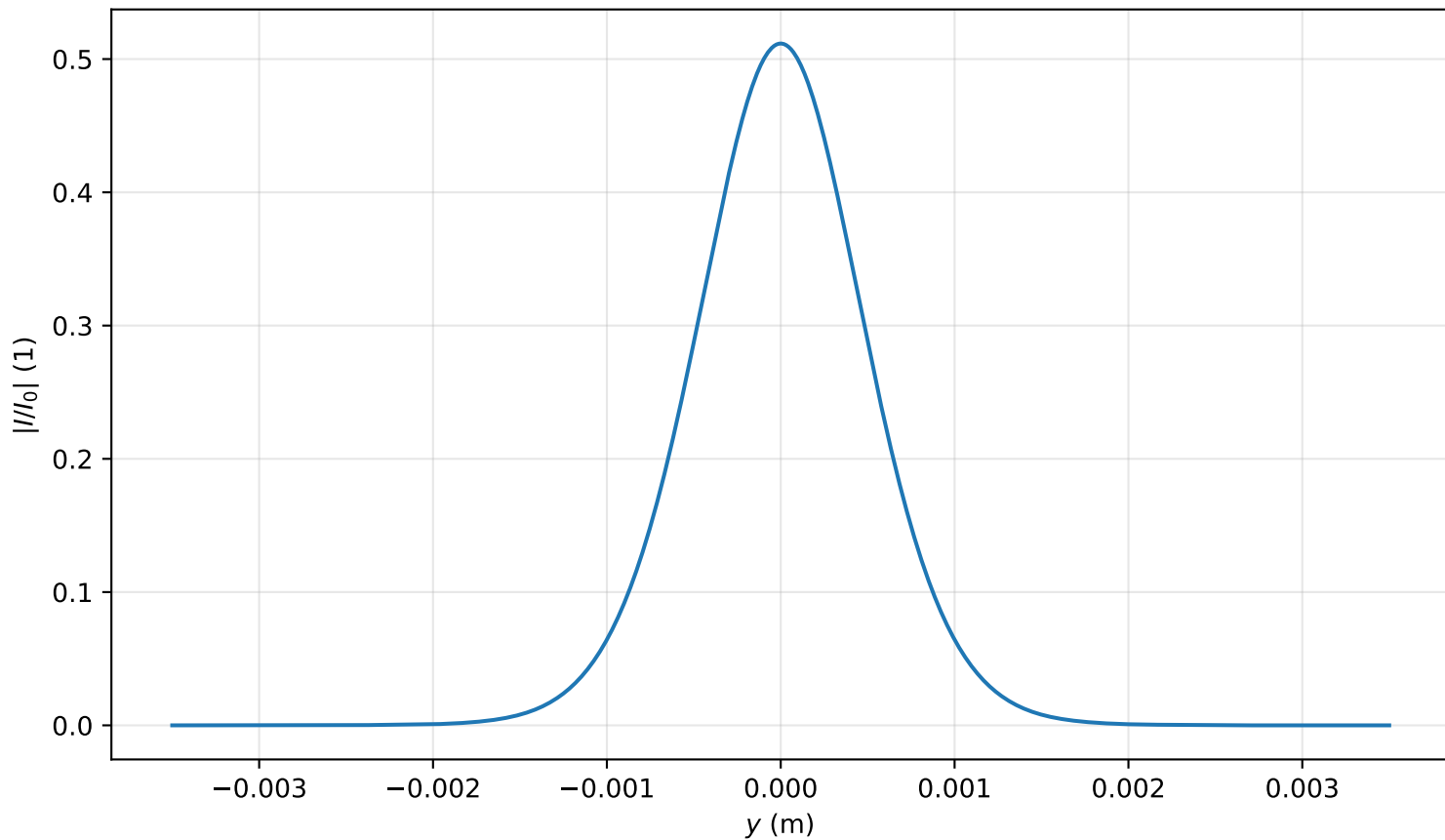
Intensity profile I(x=0, y, z=2.866)/I_0 , \text{Pin}=0.4\text{Pcr} , artificial time
